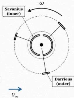
(e) Hybrid Sav.-Darrieus
