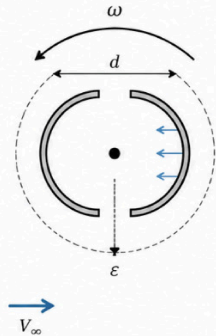
(a) Savonius S-rotor
