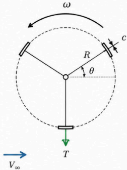
(b) H-Darrieus (straight-blade)
